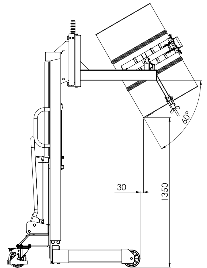
TIP OF 60°
