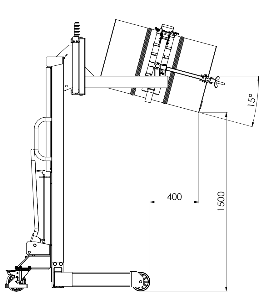
TIP OF 15°
