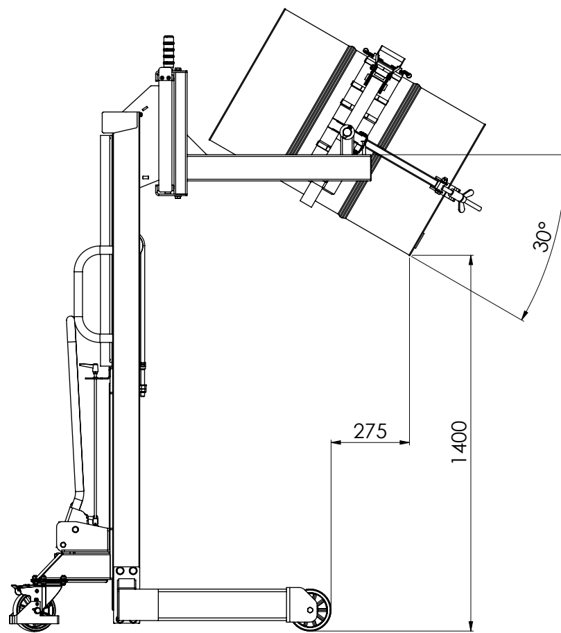
TIP OF 30°
